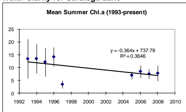
Figure 28. Annual Average Summer Chlorophyll a for Saratoga Lake
