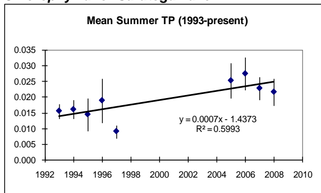
Figure 29. Annual Average Summer Total Phosphorus for Saratoga Lake
