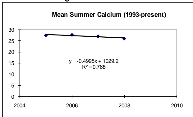
Figure 36. Annual Average Summer Calcium for Saratoga Lake
