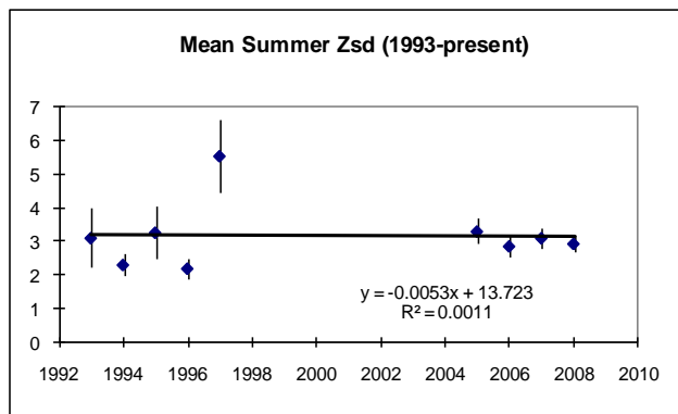
Figure 27. Annual Average Summer Water Clarity for Saratoga Lake
