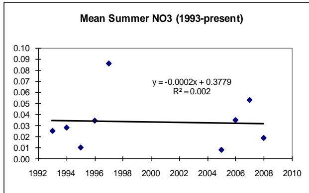
Figure 31. Annual Average Summer Nitrate for Saratoga Lake
