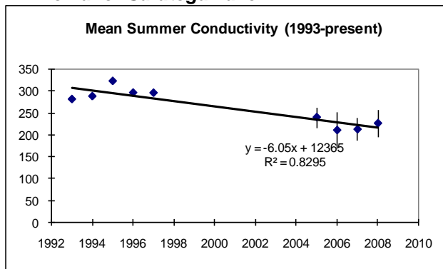
Figure 33. Annual Average Summer Conductivity for Saratoga Lake
