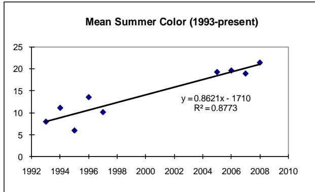
Figure 35. Annual Average Summer Color for Saratoga Lake
