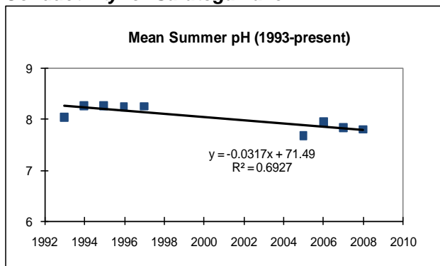
Figure 34. Annual Average Summer pH for Saratoga Lake
