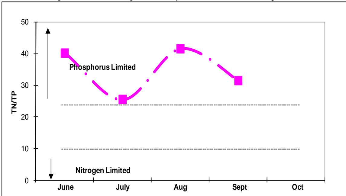
Figure 26- Nitrogen-to-Phosphorus Ratios in a Typical (Monthly Mean) Year for Saratoga Lake
