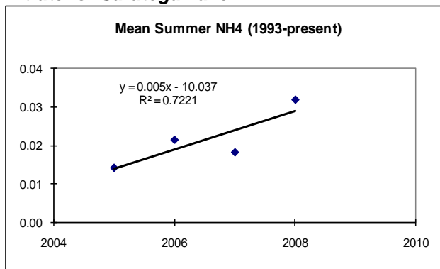
Figure 32. Annual Average Summer Ammonia for Saratoga Lake
