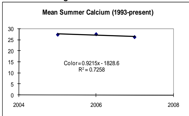
Figure 36. Annual Average Summer Calcium for Saratoga Lake
