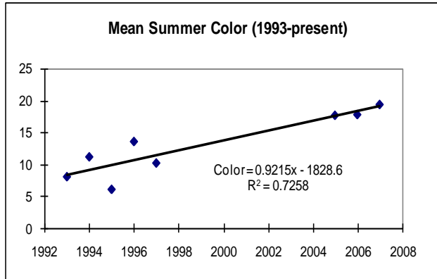
Figure 35. Annual Average Summer Color for Saratoga Lake
