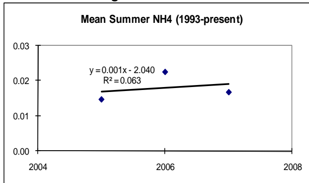
Figure 32. Annual Average Summer Ammonia for Saratoga Lake
