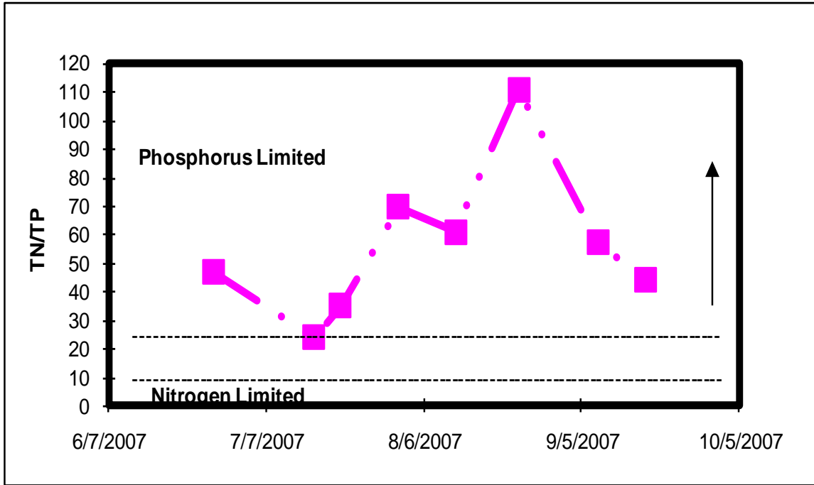
Figure 25. 2007 Nitrogen-to-Phosphorus Ratios for Saratoga Lake
