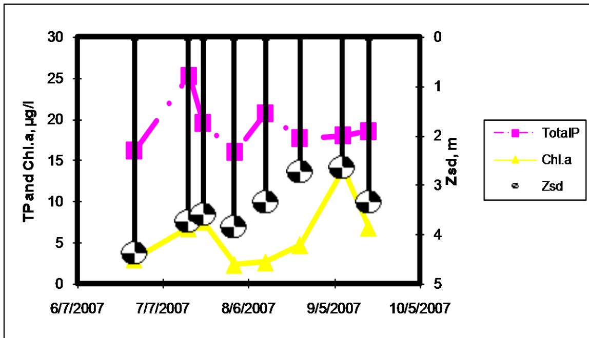
Figure 23. 2007 Eutrophication Data for Saratoga Lake
