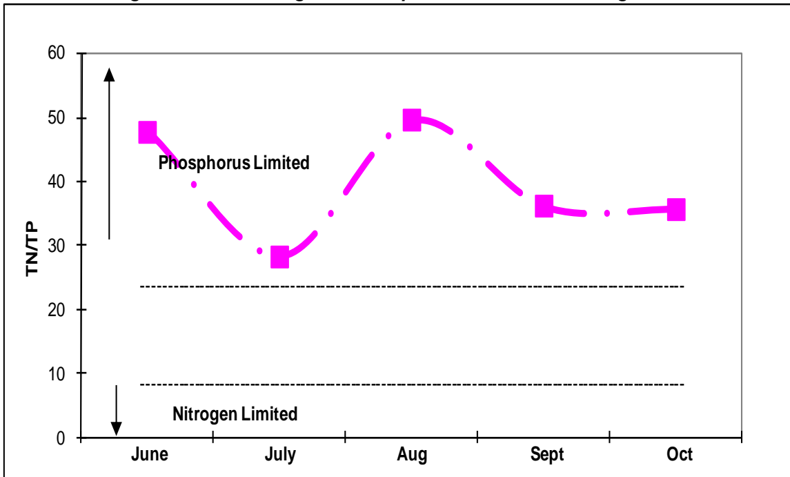
Figure 26- Nitrogen-to-Phosphorus Ratios in a Typical (Monthly Mean) Year for Saratoga Lake
