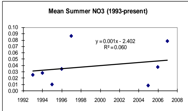
Figure 31. Annual Average Summer Nitrate for Saratoga Lake
