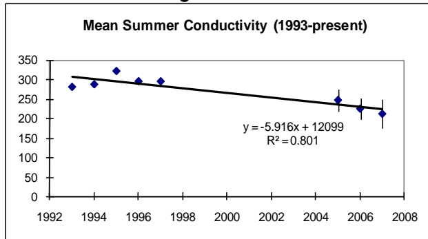
Figure 33. Annual Average Summer Conductivity for Saratoga Lake
