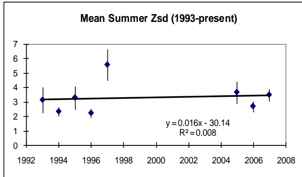
Figure 27. Annual Average Summer Water Clarity for Saratoga Lake
