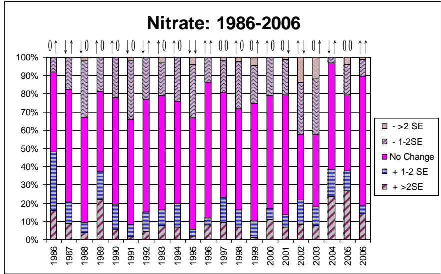
Figure 14a. Annual Change from “Normal” Nitrate in CSLAP Lakes (SE = Standard Error)
