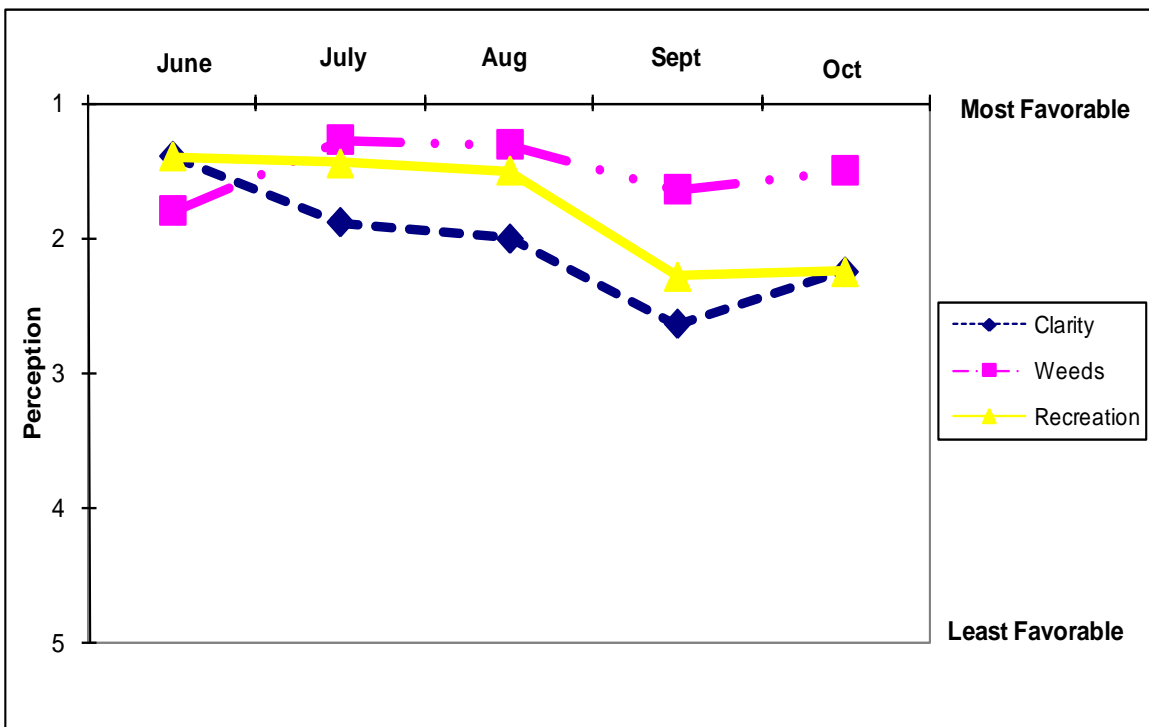
Figure 39- Lake Perception Data in a Typical (Monthly Mean) Year for Saratoga Lake
