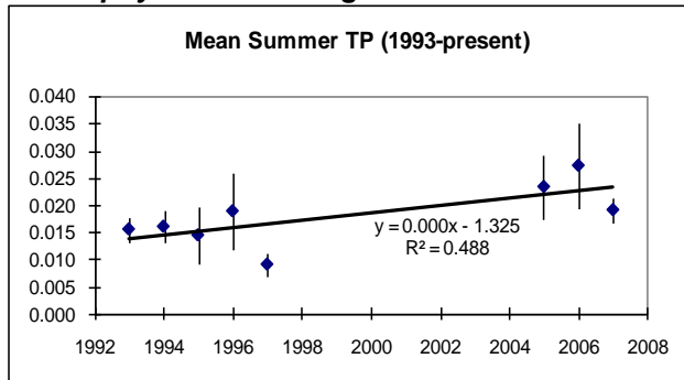
Figure 29. Annual Average Summer Total Phosphorus for Saratoga Lake
