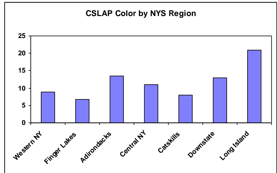
Figure 12b. Color in CSLAP Lakes by NYS Region
