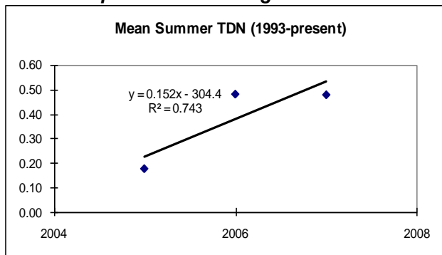
Figure 30. Annual Average Summer Total Nitrogen for Saratoga Lake
